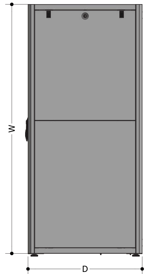
Side View
