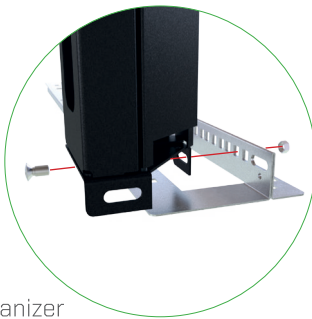
Organizer Mounting Detail
